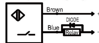
Relay Load Source(PNP) Wiring diagram
